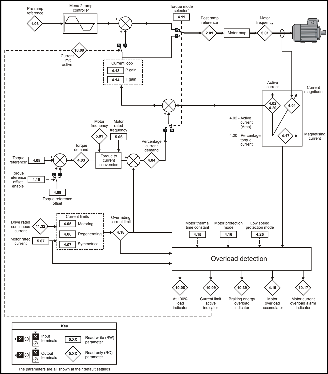
5.6.3 Parameter descriptions Parameter descriptions: Open-loop Figure 5-5 Menu 4 Open-loop logic diagram
