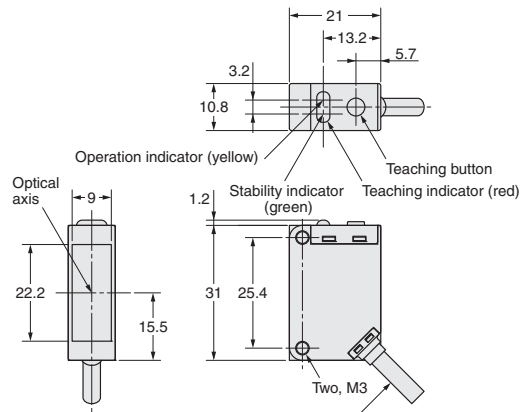
M12 Pre-wired Connector (E3ZM-□□□-M1J)
